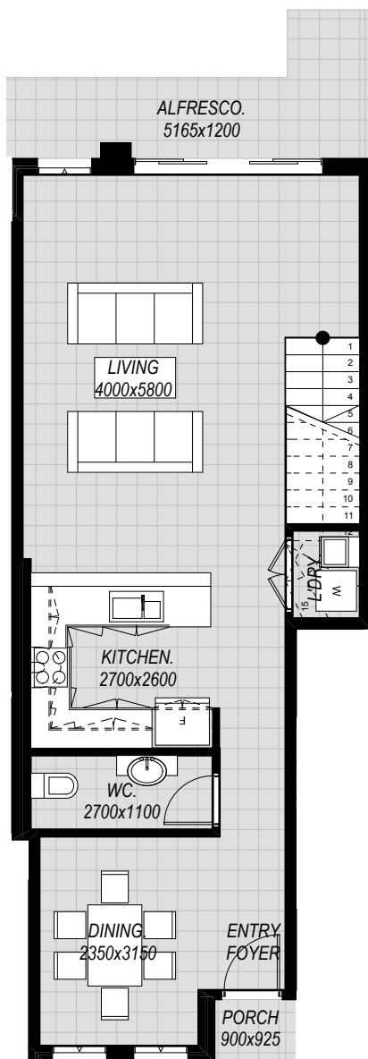
GROUND FLOOR SCALE 1:100 (A4)
