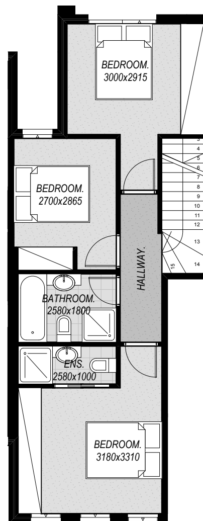
FIRST FLOOR SCALE 1:100 (A4)
