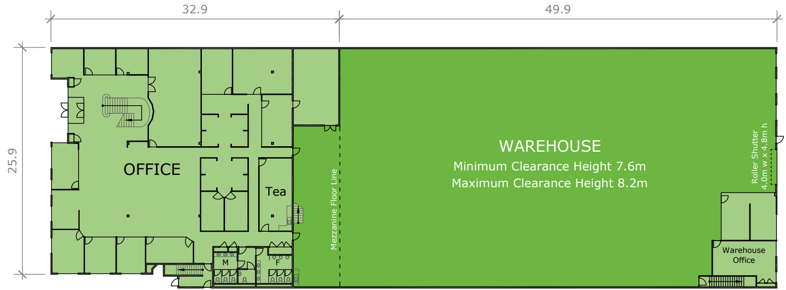
GROUND FLOOR
